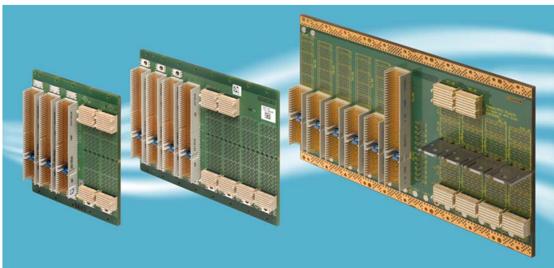
Sample Hybrid CompactPCI® &amp; CompactPCI® Serial Backplanes
