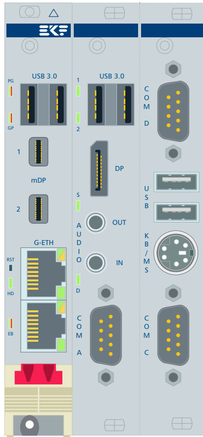
PC4-PRESTO Dual - mDP PCS-BALLET RS-232 C32-FIO
